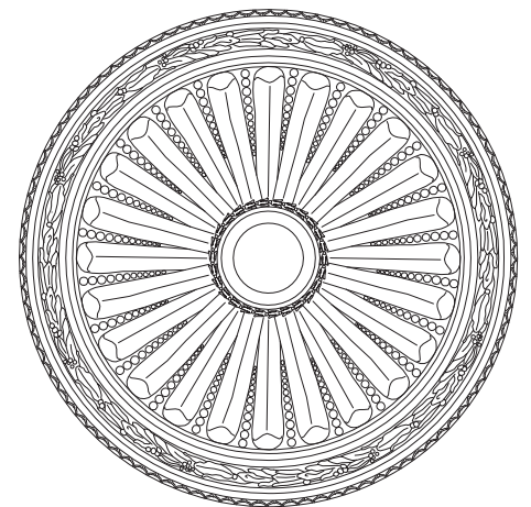
PLAS 849 TONGUE & PEARL ROSETTE 28-1/4" DIAMETER x 2-1/2" DEPTH 4" DIAMETER AT CENTER HOLE 1/2" DEPTH AT CENTER HOLE 5-3/8" DIA. FLAT AREA AT CENTER 30 LBS TOTAL WEIGHT
