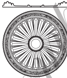
PLAS 849 TONGUE & PEARL ROSETTE 28-1/4" DIAMETER x 2-1/2" DEPTH 4" DIAMETER AT CENTER HOLE 1/2" DEPTH AT CENTER HOLE 5-3/8" DIA. FLAT AREA AT CENTER 30 LBS TOTAL WEIGHT
