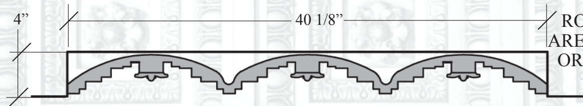
PROFILE SCALE: 1/4" = 1"
