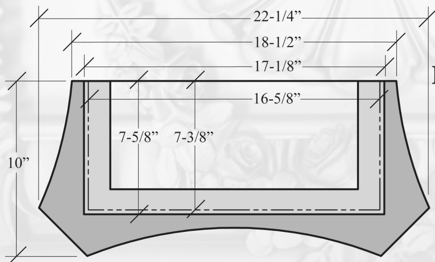
PROFILE SCALE: 3/16" = 1"
